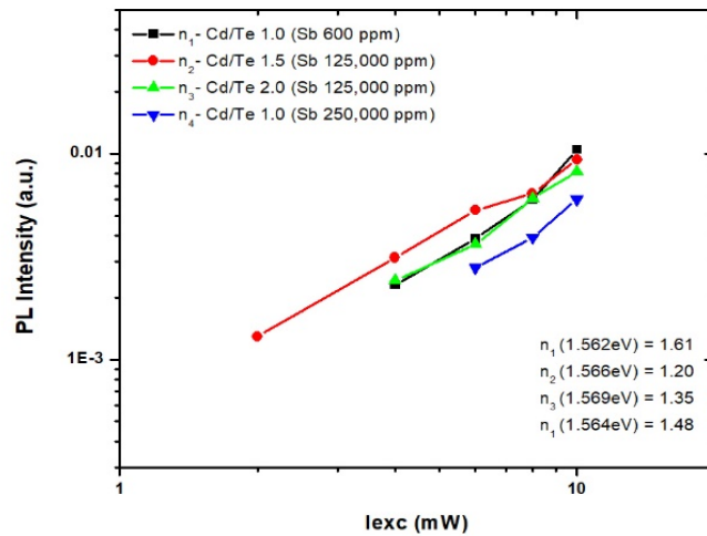
Figure 22 The PL intensity of selected bands vs. laser excitation power.
