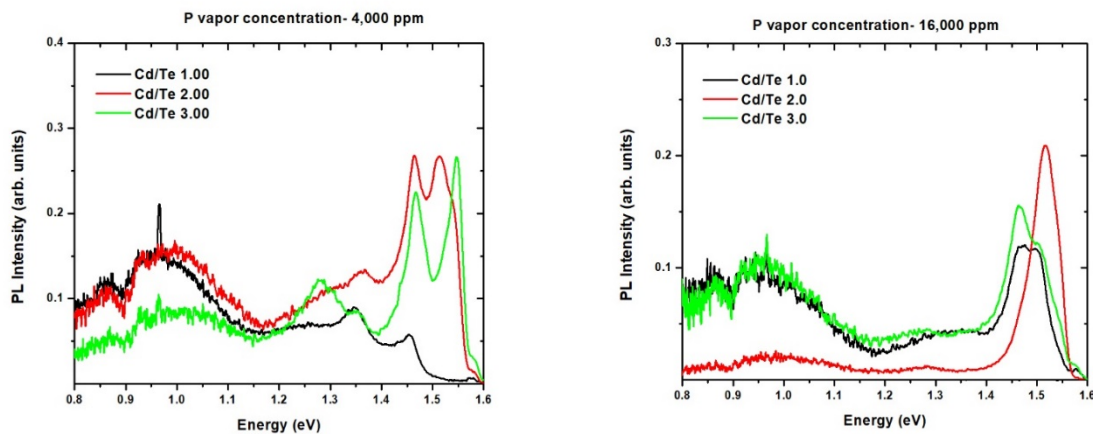
Figure 26 The PL spectra for the two concentrations of P as a function of Cd/Te ratios.
