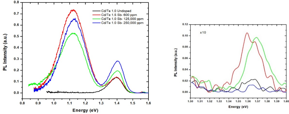
Figure 21 The PL spectra of all CdTe films, including CdTe:Sb and the undoped (as-deposited) film.
